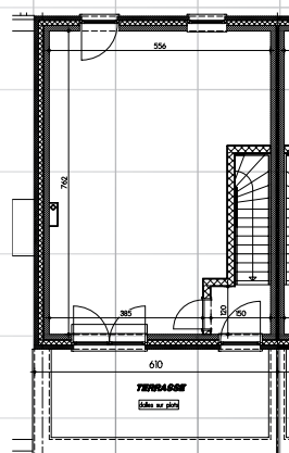
Combles
